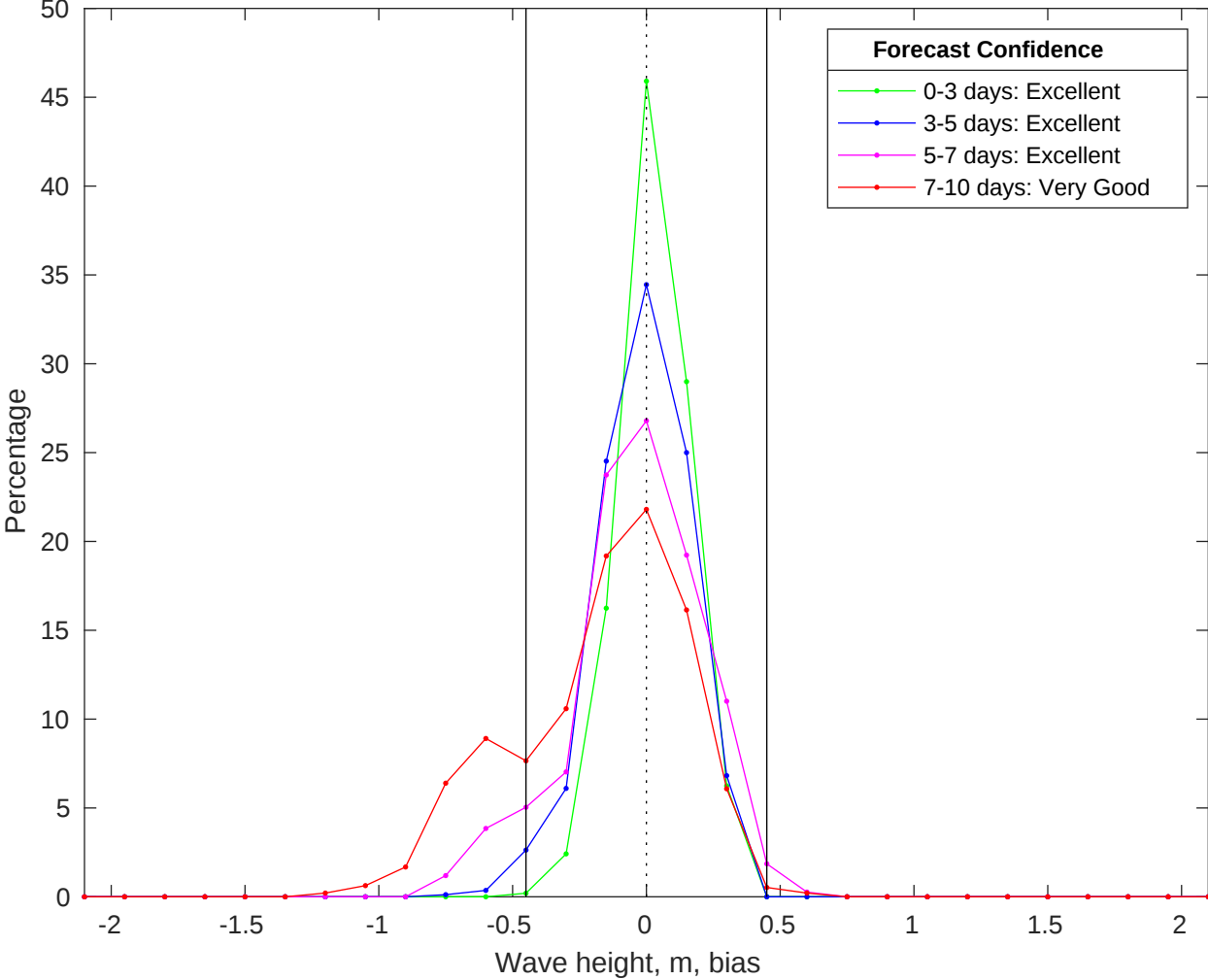
NDBC 41040 vs CMEMS Waves Bias Histogram: 27-Jun-2025
