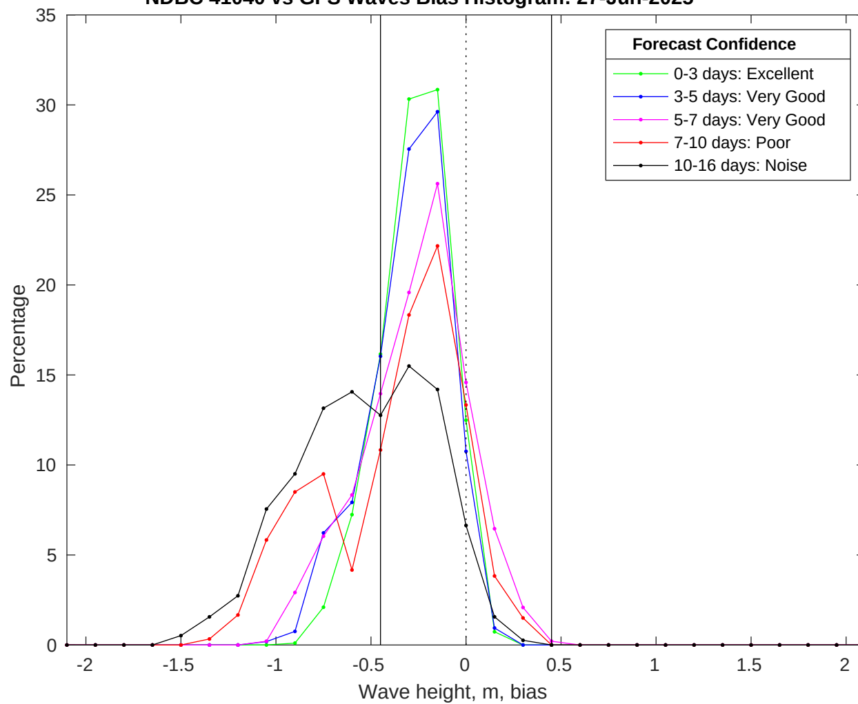
NDBC 41040 vs GFS Waves Bias Histogram: 27-Jun-2025
