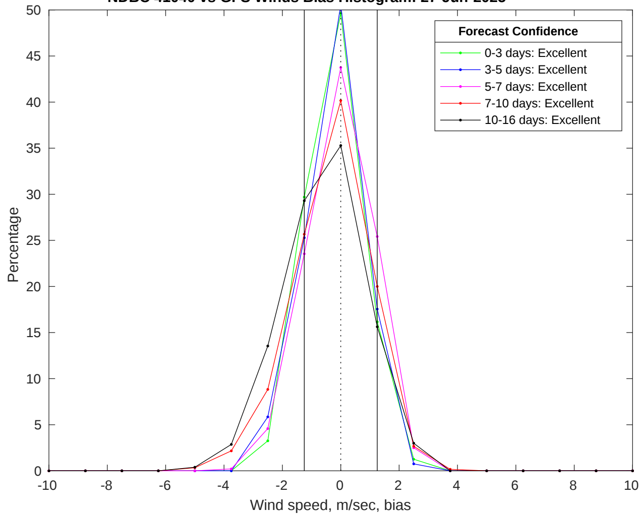
NDBC 41040 vs GFS Winds Bias Histogram: 27-Jun-2025
