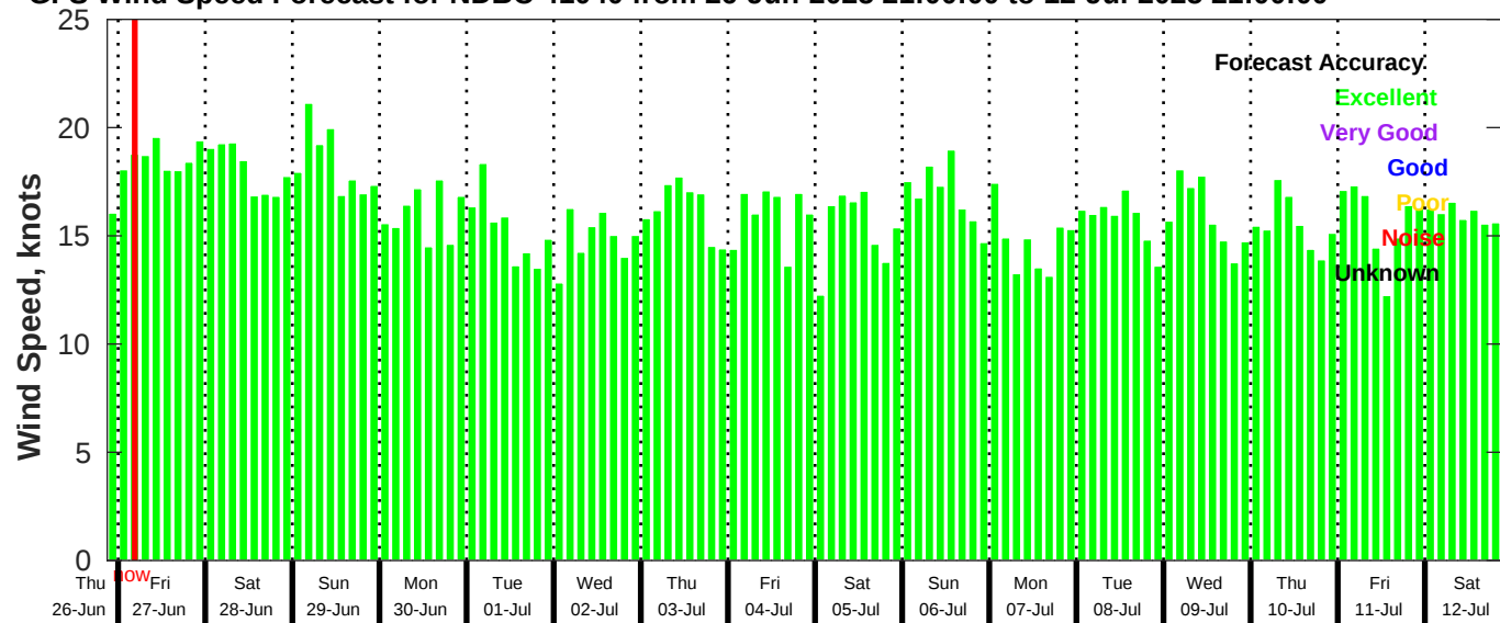
GFS Wind Speed Forecast for NDBC 41040 from 26-Jun-2025 21:00:00 to 12-Jul-2025 21:00:00
