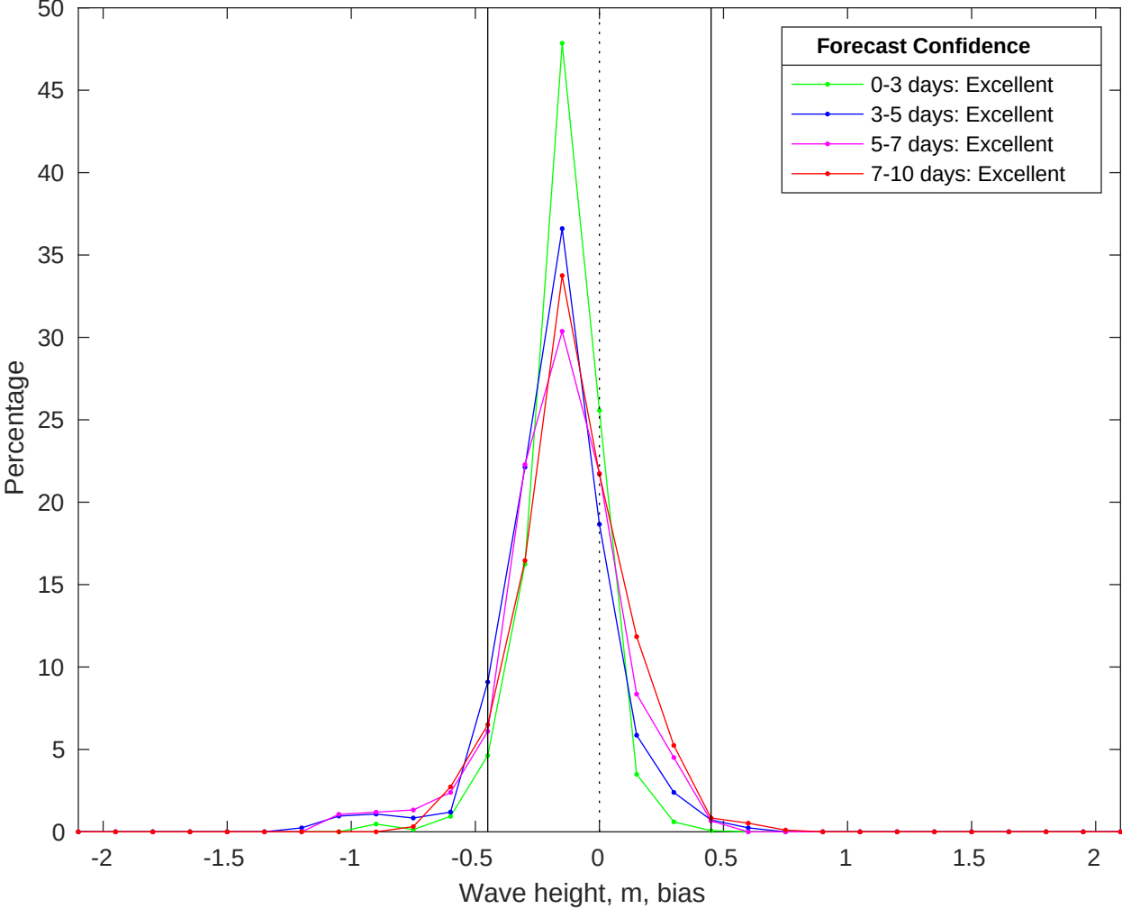
NDBC 42019 vs CMEMS Waves Bias Histogram: 27-Jun-2025
