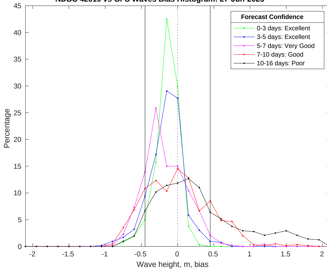
NDBC 42019 vs GFS Waves Bias Histogram: 27-Jun-2025
