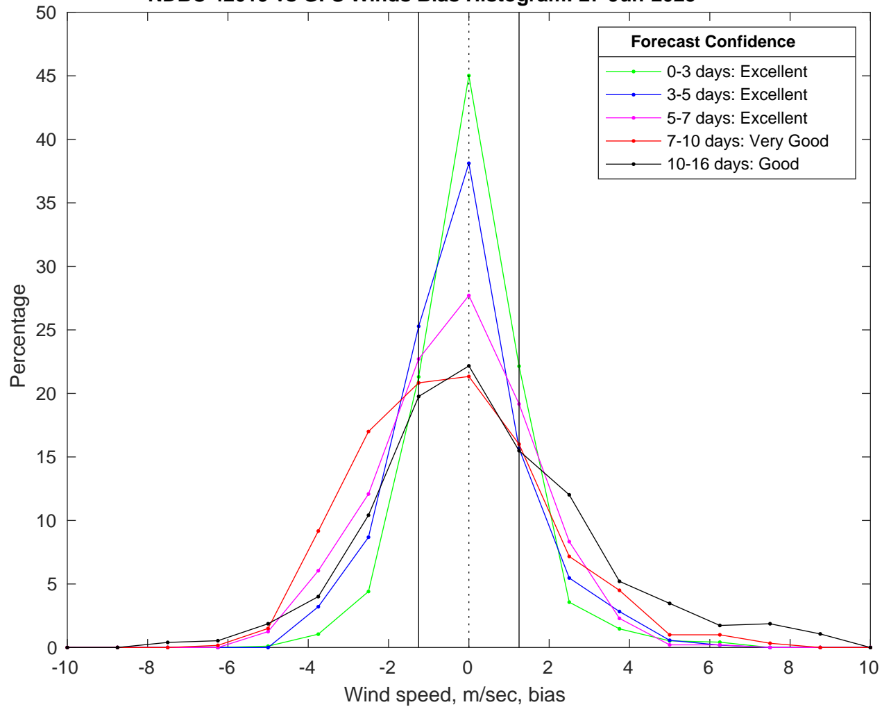
NDBC 42019 vs GFS Winds Bias Histogram: 27-Jun-2025
