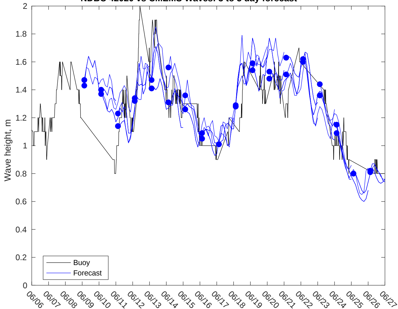
NDBC 42020 vs CMEMS Waves: 3 to 5 day forecast
