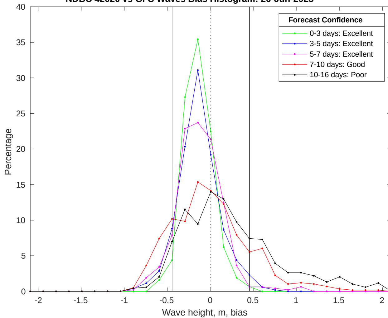
NDBC 42020 vs GFS Waves Bias Histogram: 26-Jun-2025
