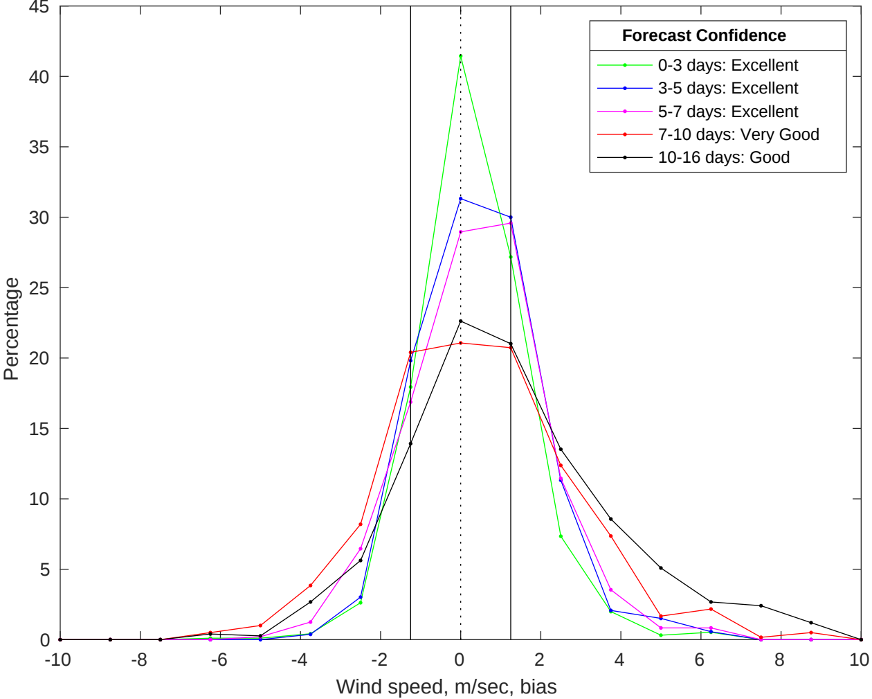
NDBC 42020 vs GFS Winds Bias Histogram: 27-Jun-2025
