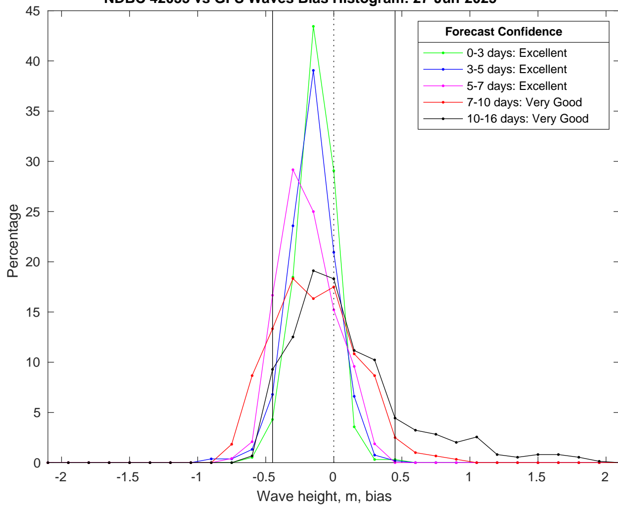
NDBC 42035 vs GFS Waves Bias Histogram: 27-Jun-2025
