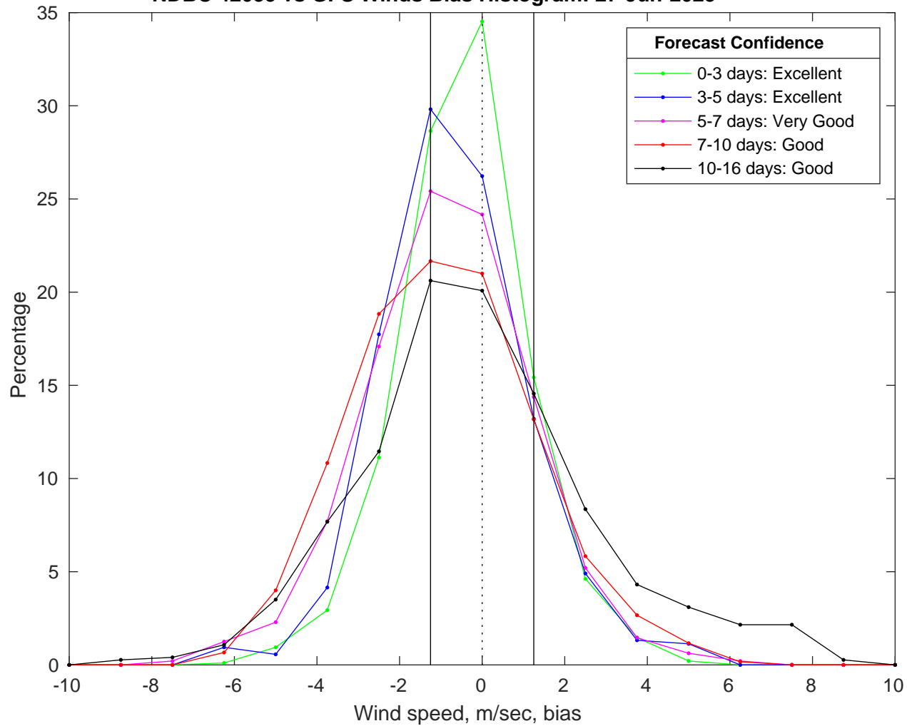
NDBC 42035 vs GFS Winds Bias Histogram: 27-Jun-2025
