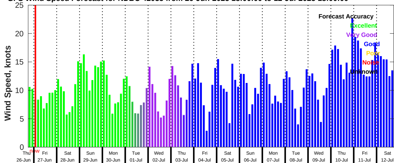
GFS Wind Speed Forecast for NDBC 42035 from 26-Jun-2025 18:00:00 to 12-Jul-2025 18:00:00
