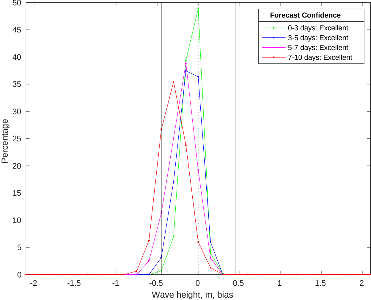
NDBC 42036 vs CMEMS Waves Bias Histogram: 27-Jun-2025
