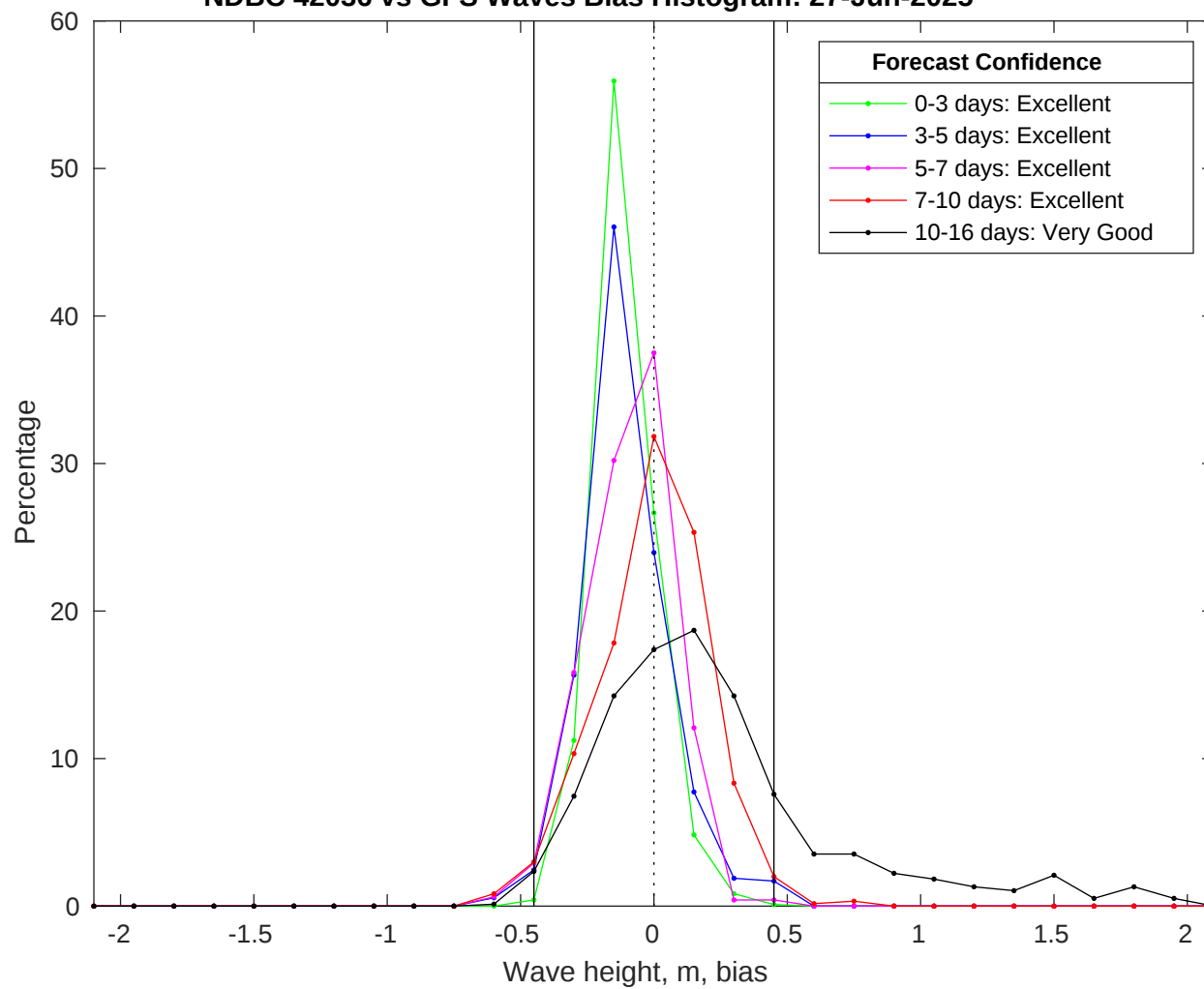
NDBC 42036 vs GFS Waves Bias Histogram: 27-Jun-2025
