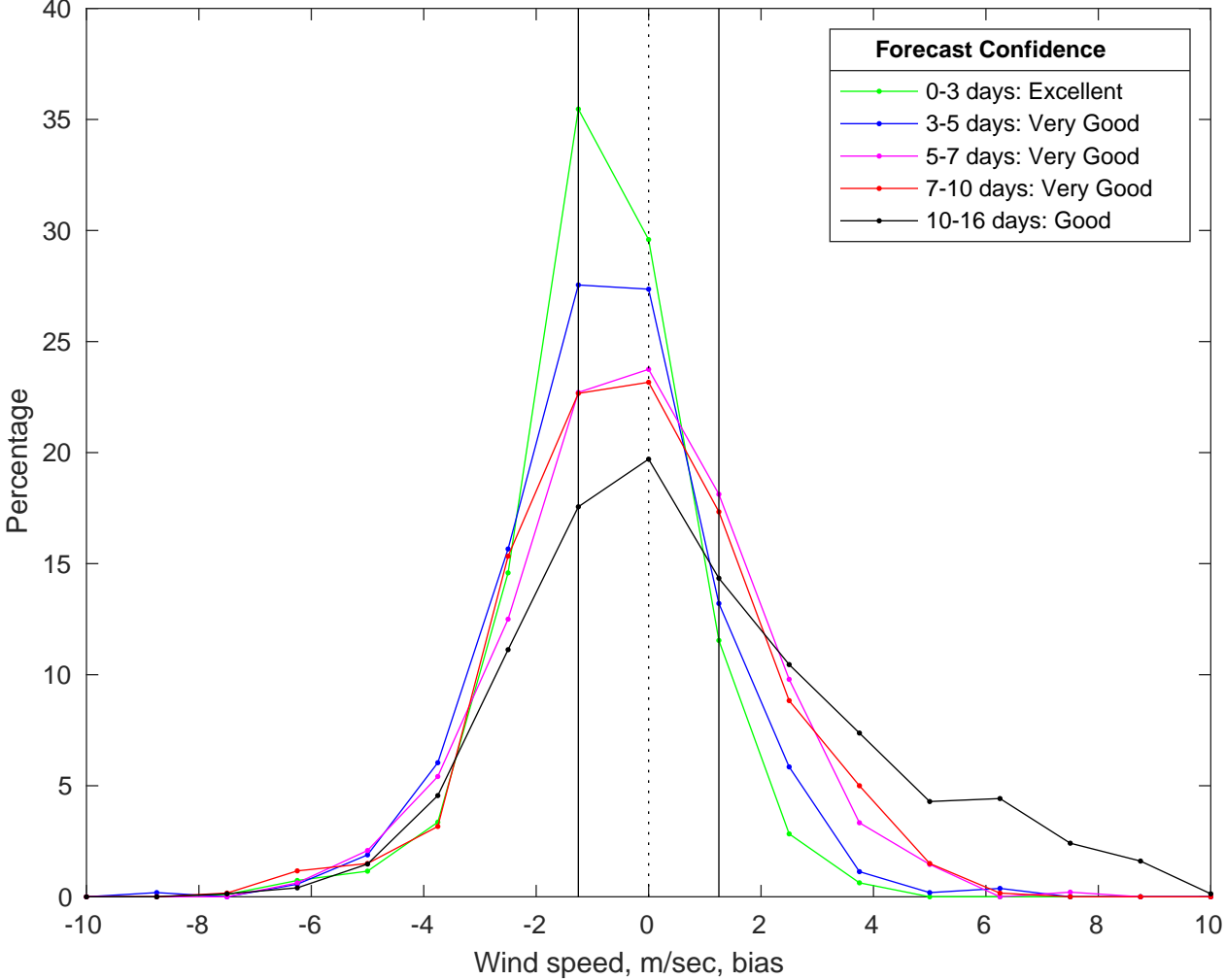
NDBC 42040 vs GFS Winds Bias Histogram: 27-Jun-2025
