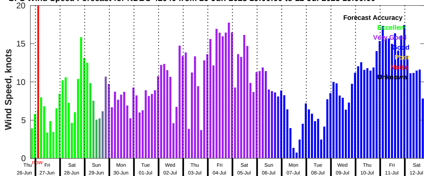
GFS Wind Speed Forecast for NDBC 42040 from 26-Jun-2025 19:00:00 to 12-Jul-2025 19:00:00
