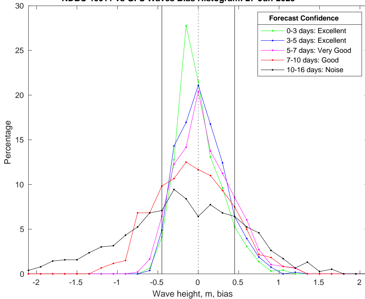
NDBC 46011 vs GFS Waves Bias Histogram: 27-Jun-2025
