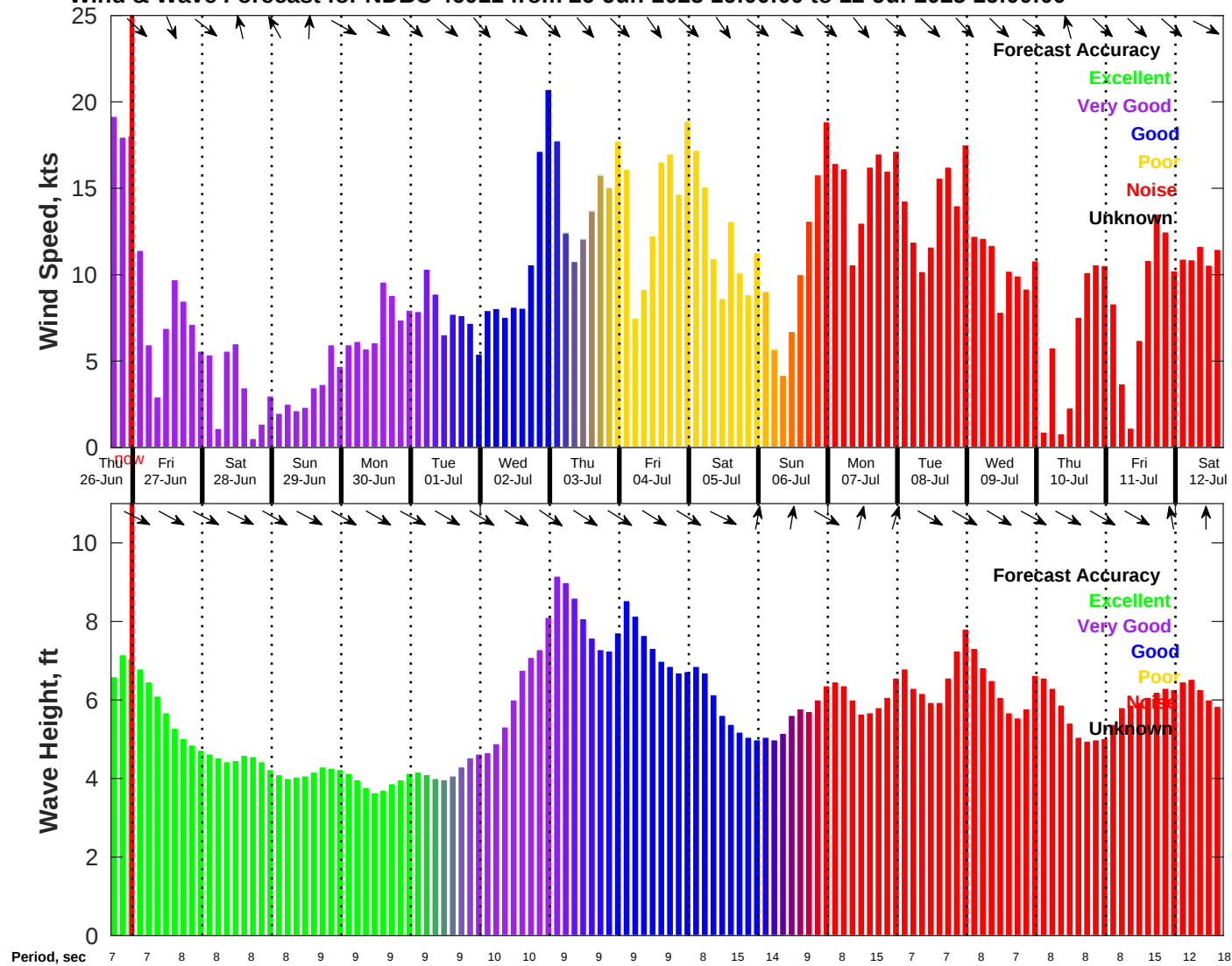
Wind & Wave Forecast for NDBC 46011 from 26-Jun-2025 16:00:00 to 12-Jul-2025 16:00:00
