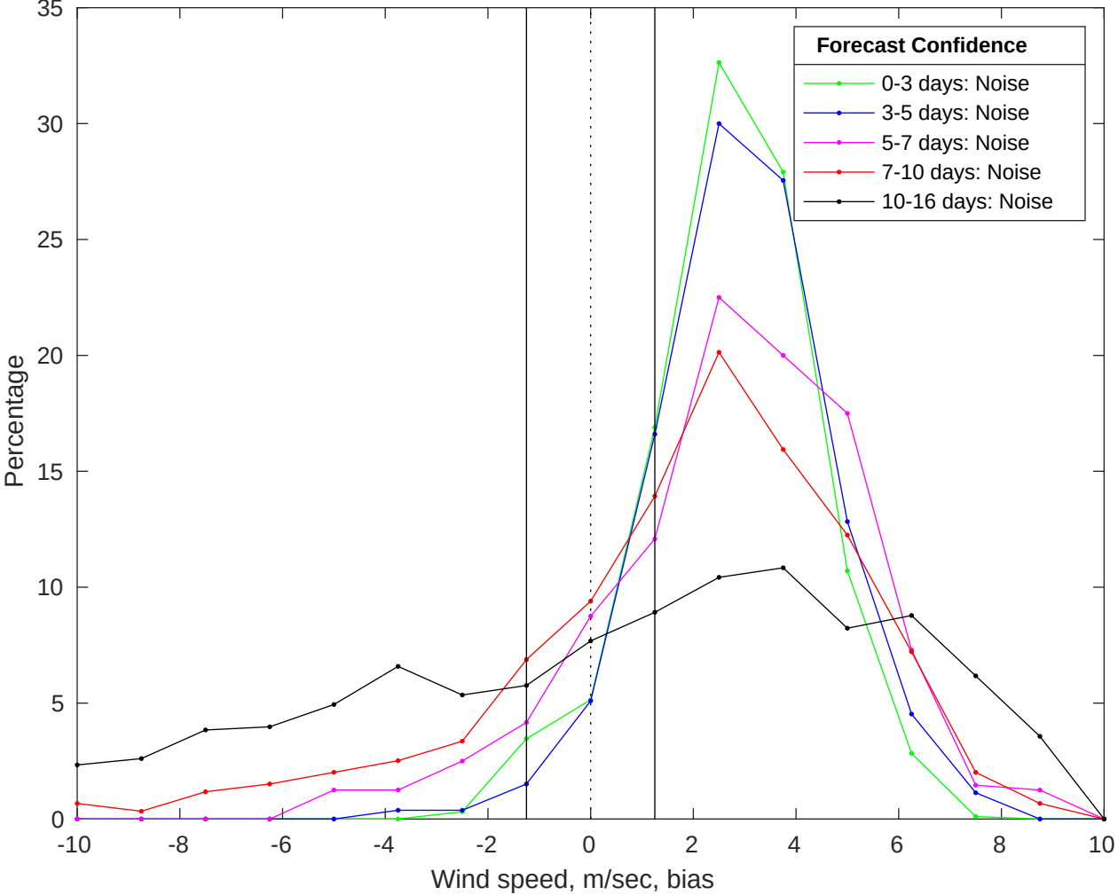
NDBC 46028 vs GFS Winds Bias Histogram: 27-Jun-2025
