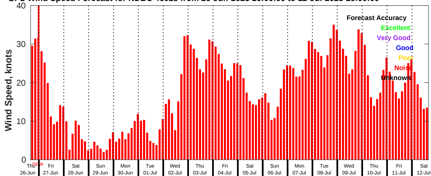
GFS Wind Speed Forecast for NDBC 46028 from 26-Jun-2025 16:00:00 to 12-Jul-2025 16:00:00
