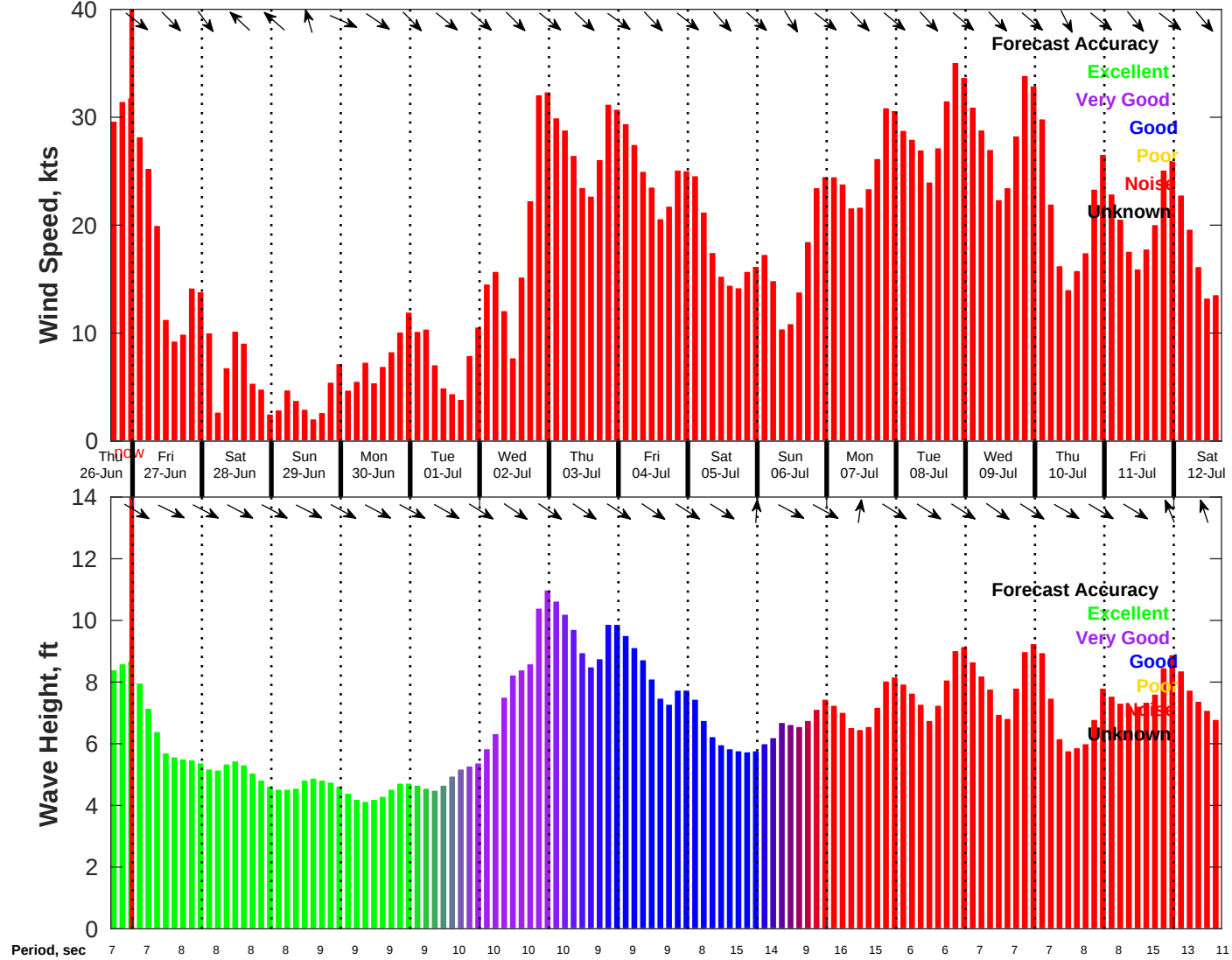
Wind & Wave Forecast for NDBC 46028 from 26-Jun-2025 16:00:00 to 12-Jul-2025 16:00:00
