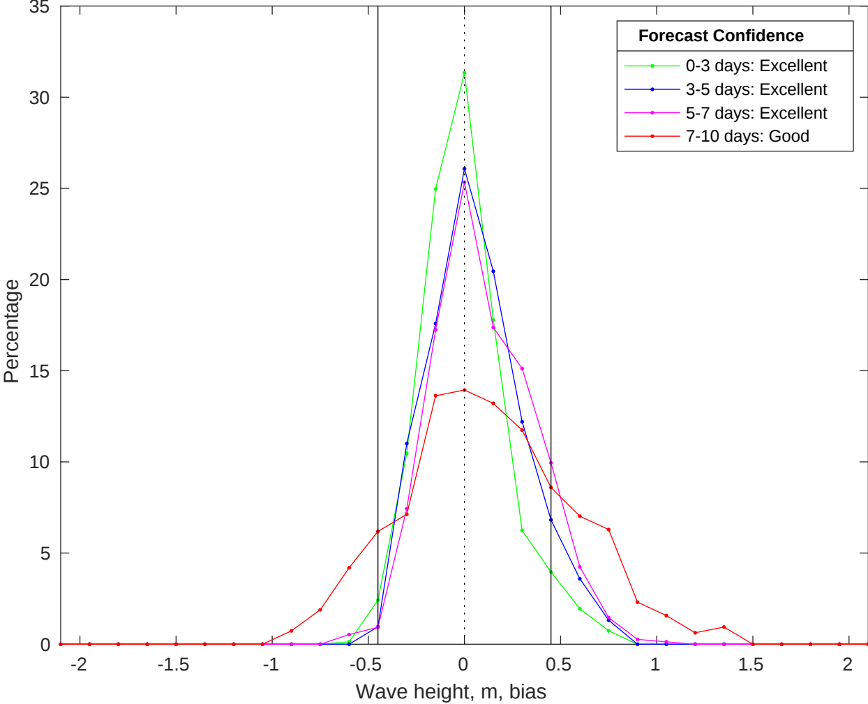
NDBC 46054 vs CMEMS Waves Bias Histogram: 27-Jun-2025
