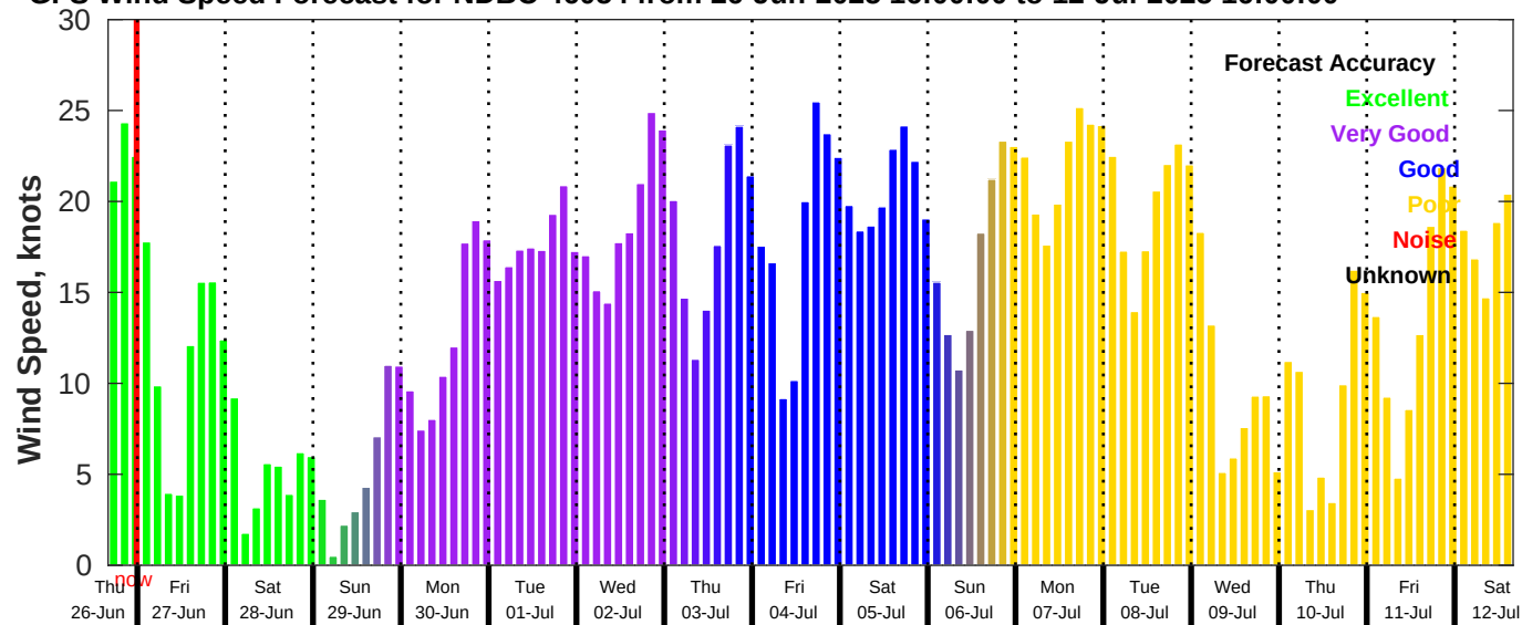
GFS Wind Speed Forecast for NDBC 46054 from 26-Jun-2025 16:00:00 to 12-Jul-2025 16:00:00
