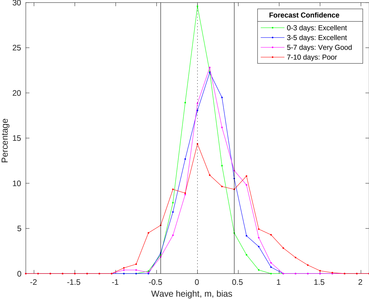
NDBC 46069 vs CMEMS Waves Bias Histogram: 27-Jun-2025
