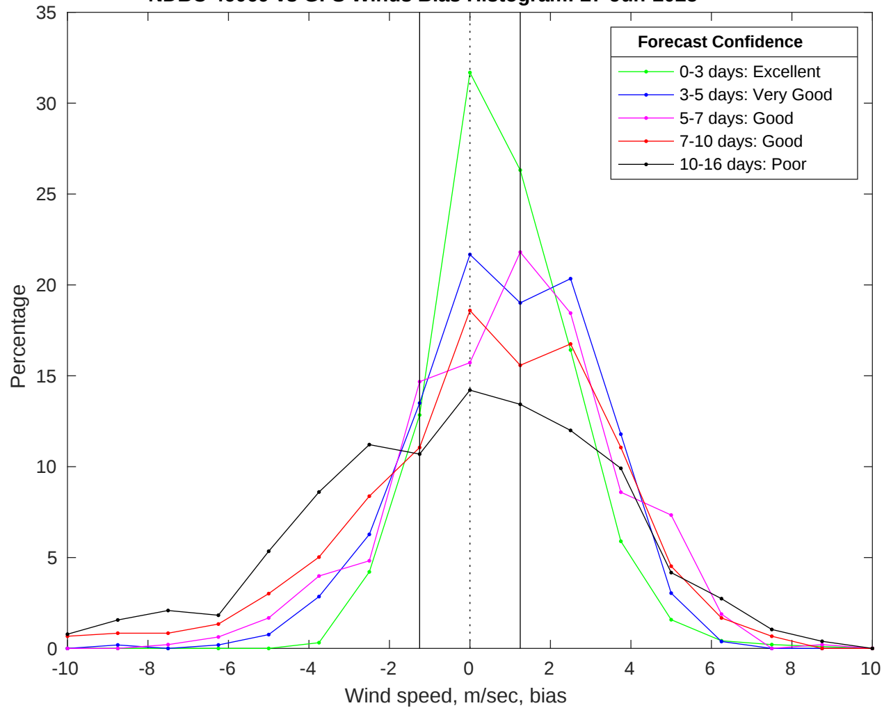
NDBC 46069 vs GFS Winds Bias Histogram: 27-Jun-2025
