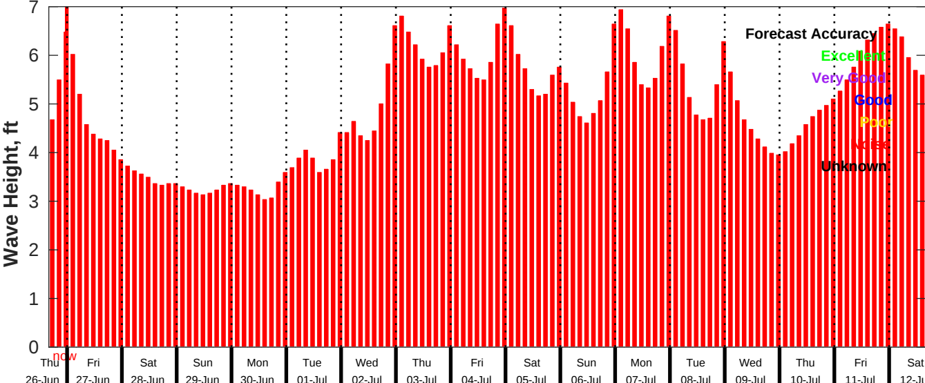
GFS Wave Forecast for NDBC 46069 from 26-Jun-2025 16:00:00 to 12-Jul-2025 16:00:00
