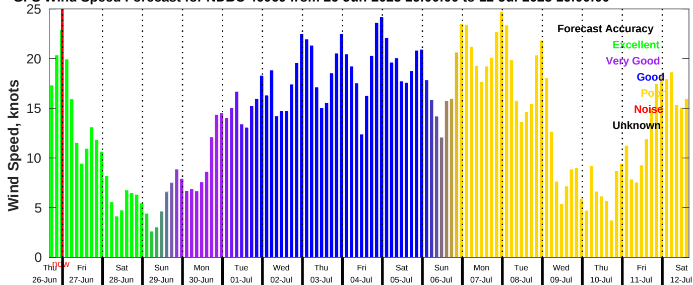
GFS Wind Speed Forecast for NDBC 46069 from 26-Jun-2025 16:00:00 to 12-Jul-2025 16:00:00
