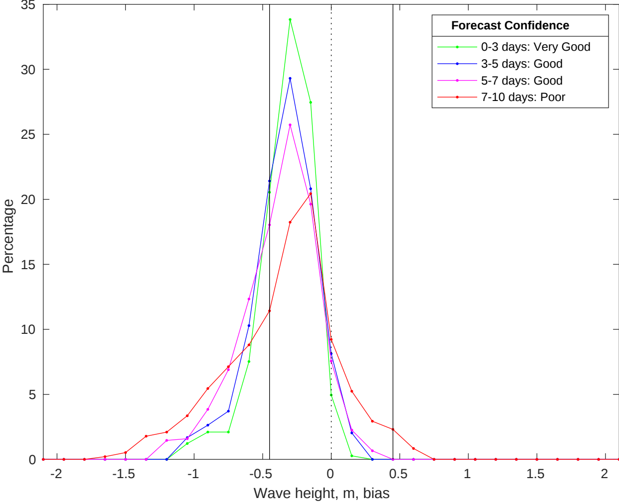
NDBC 51209 vs CMEMS Waves Bias Histogram: 27-Jun-2025
