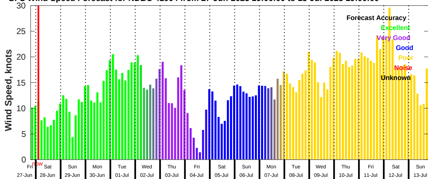
GFS Wind Speed Forecast for NDBC 41004 from 27-Jun-2025 19:00:00 to 13-Jul-2025 19:00:00
