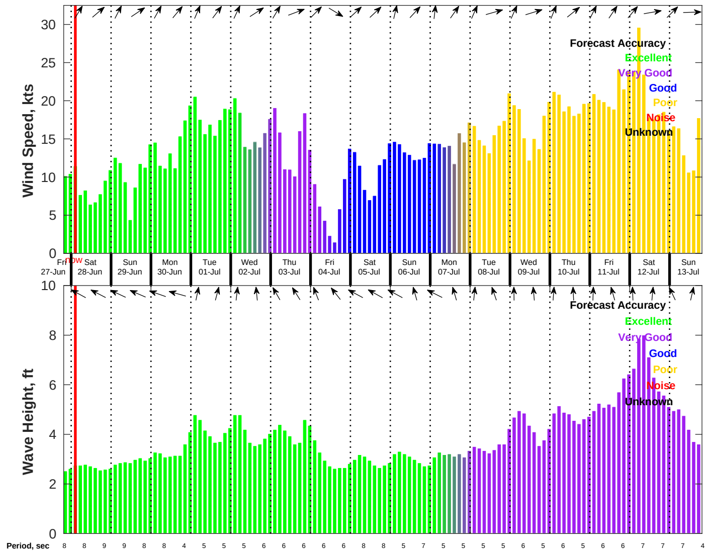
Wind & Wave Forecast for NDBC 41004 from 27-Jun-2025 19:00:00 to 13-Jul-2025 19:00:00
