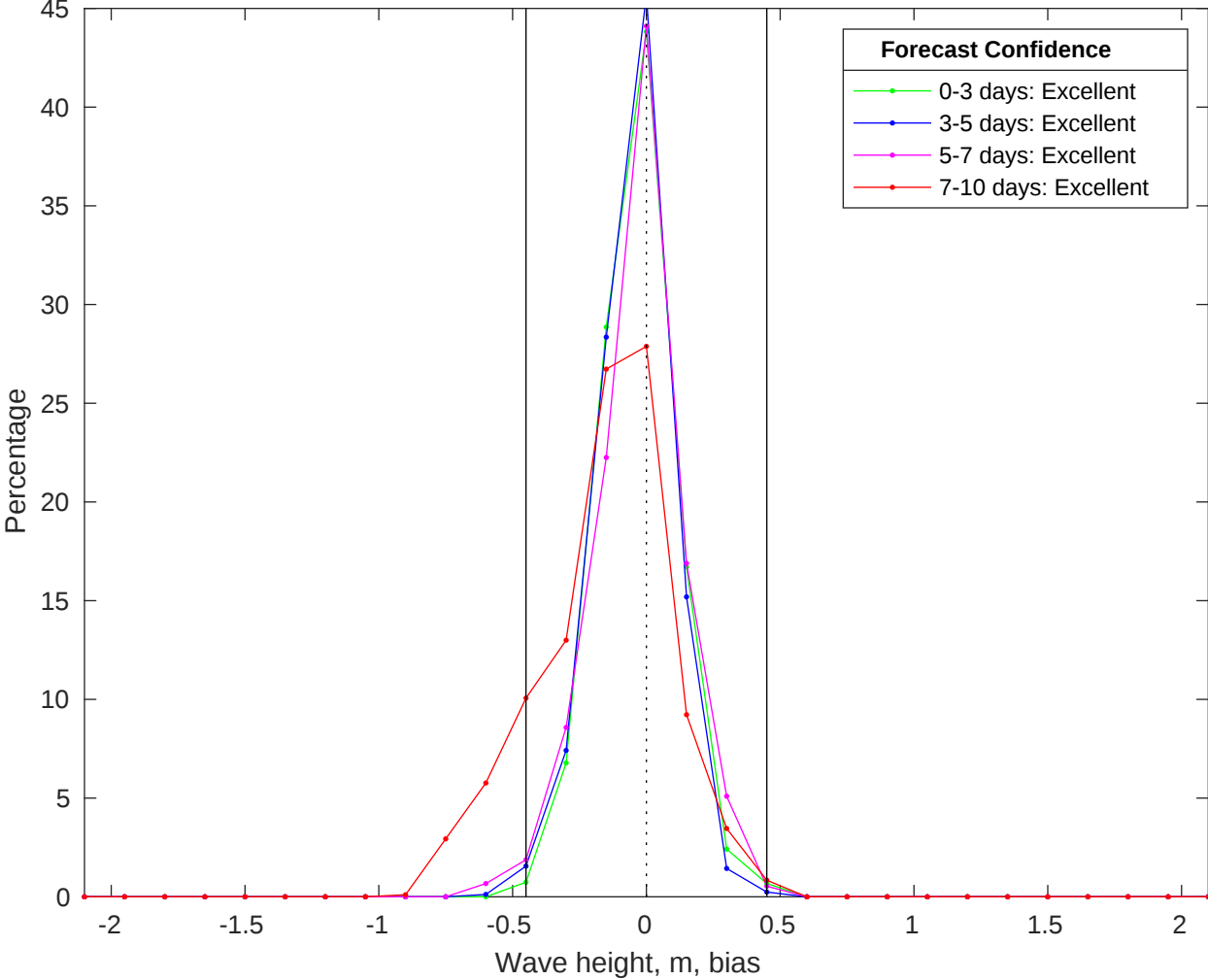
NDBC 41013 vs CMEMS Waves Bias Histogram: 28-Jun-2025
