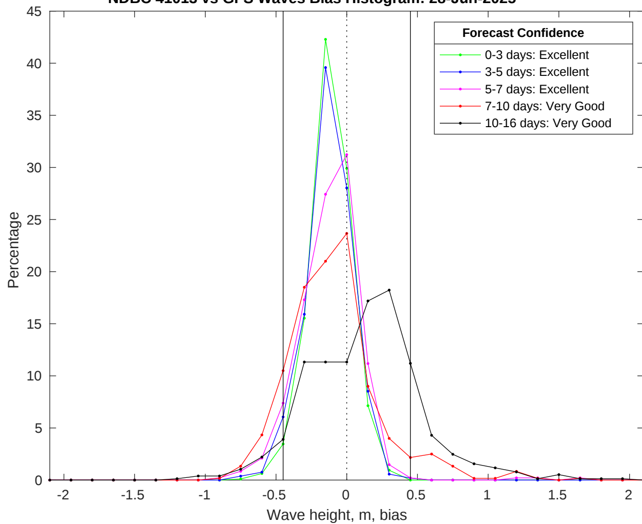
NDBC 41013 vs GFS Waves Bias Histogram: 28-Jun-2025
