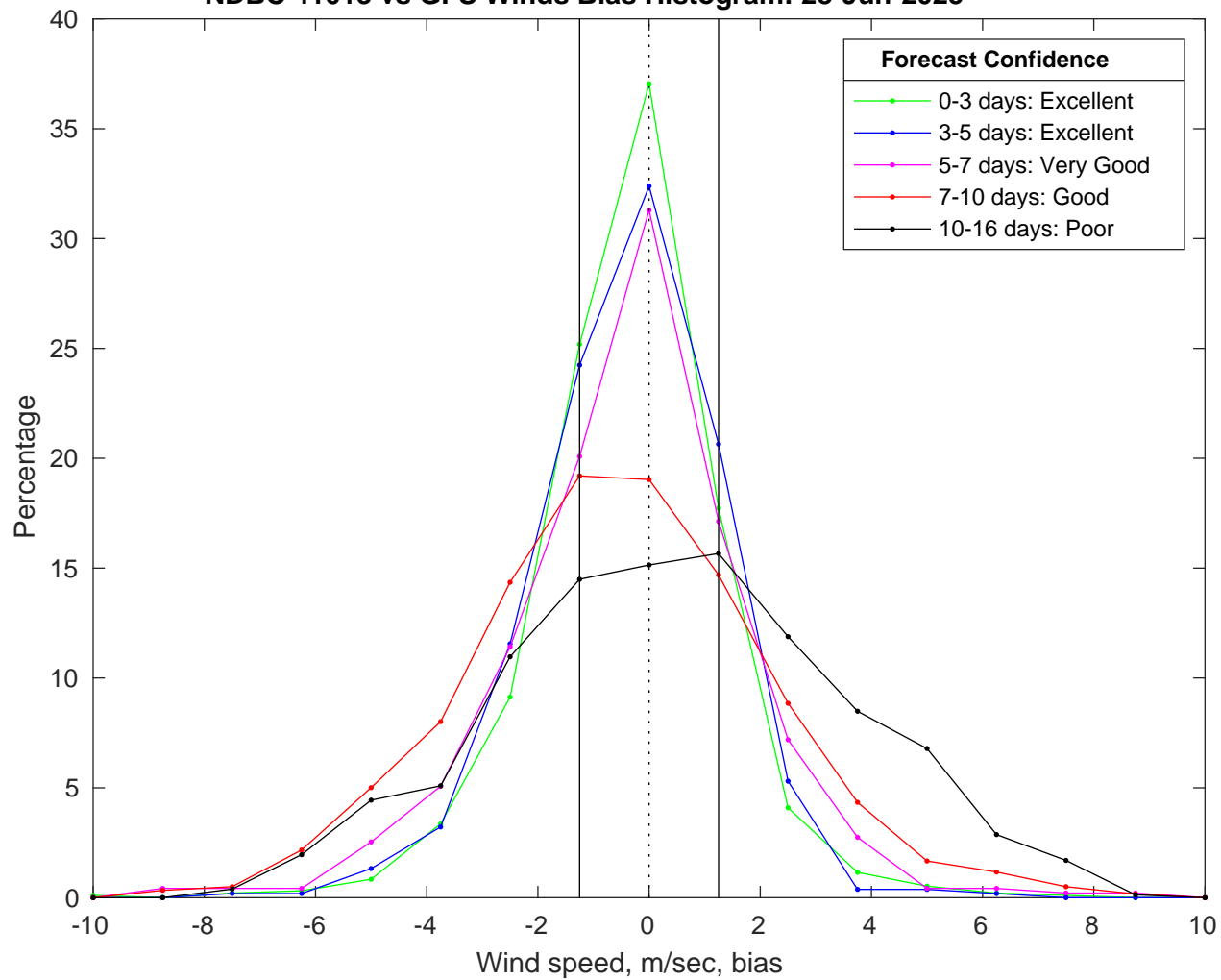
NDBC 41013 vs GFS Winds Bias Histogram: 28-Jun-2025
