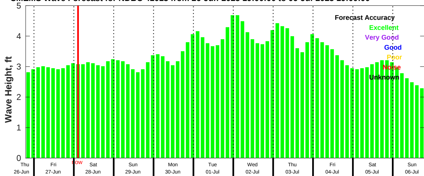
CMEMS Wave Forecast for NDBC 41013 from 26-Jun-2025 19:00:00 to 06-Jul-2025 19:00:00
