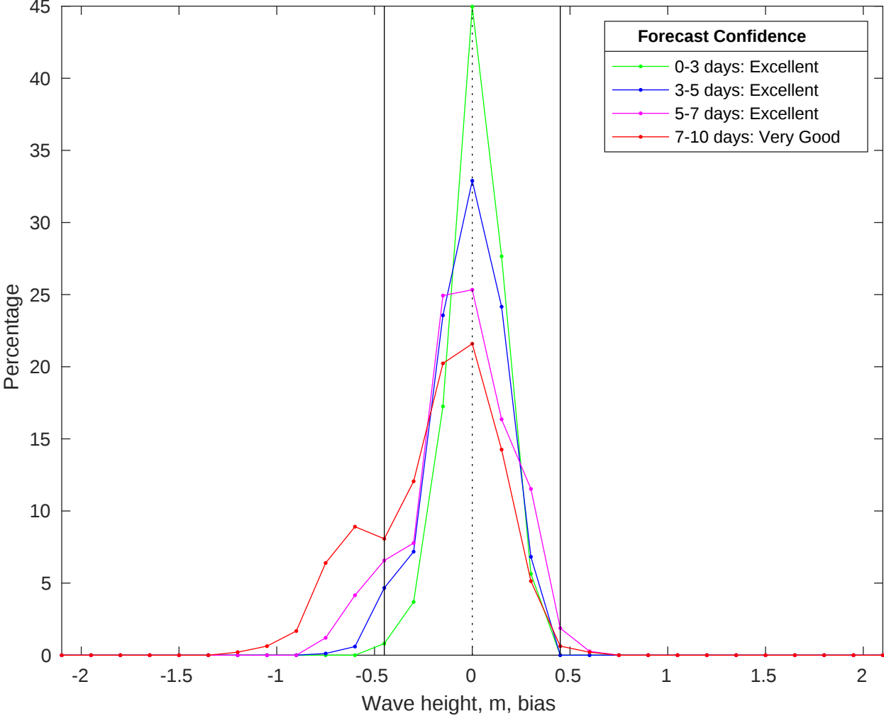
NDBC 41040 vs CMEMS Waves Bias Histogram: 28-Jun-2025
