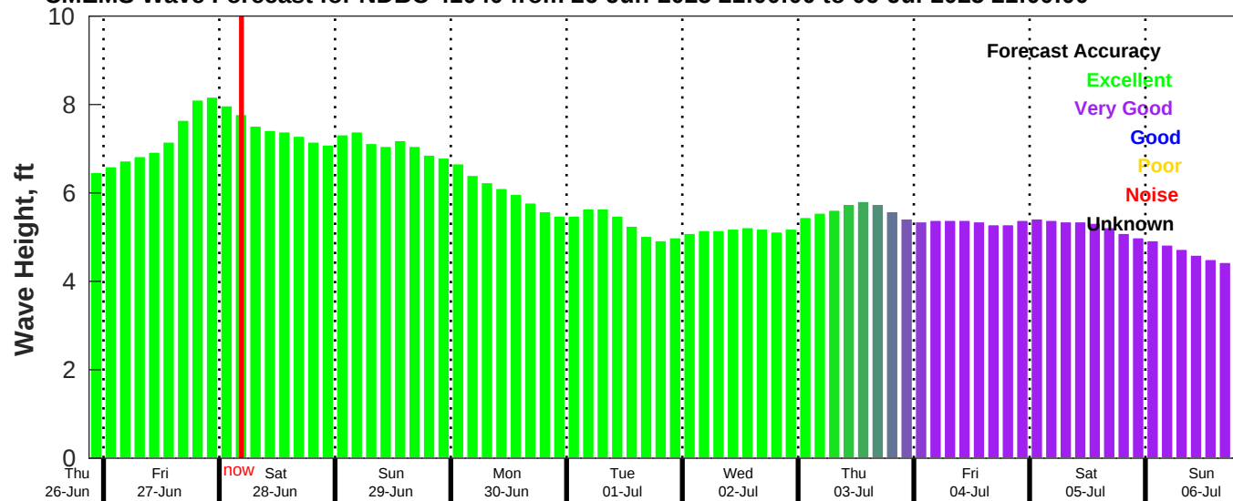
CMEMS Wave Forecast for NDBC 41040 from 26-Jun-2025 21:00:00 to 06-Jul-2025 21:00:00
