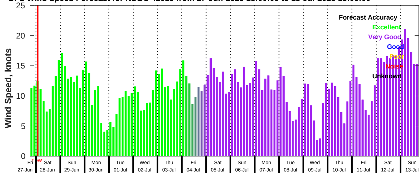
GFS Wind Speed Forecast for NDBC 42019 from 27-Jun-2025 18:00:00 to 13-Jul-2025 18:00:00
