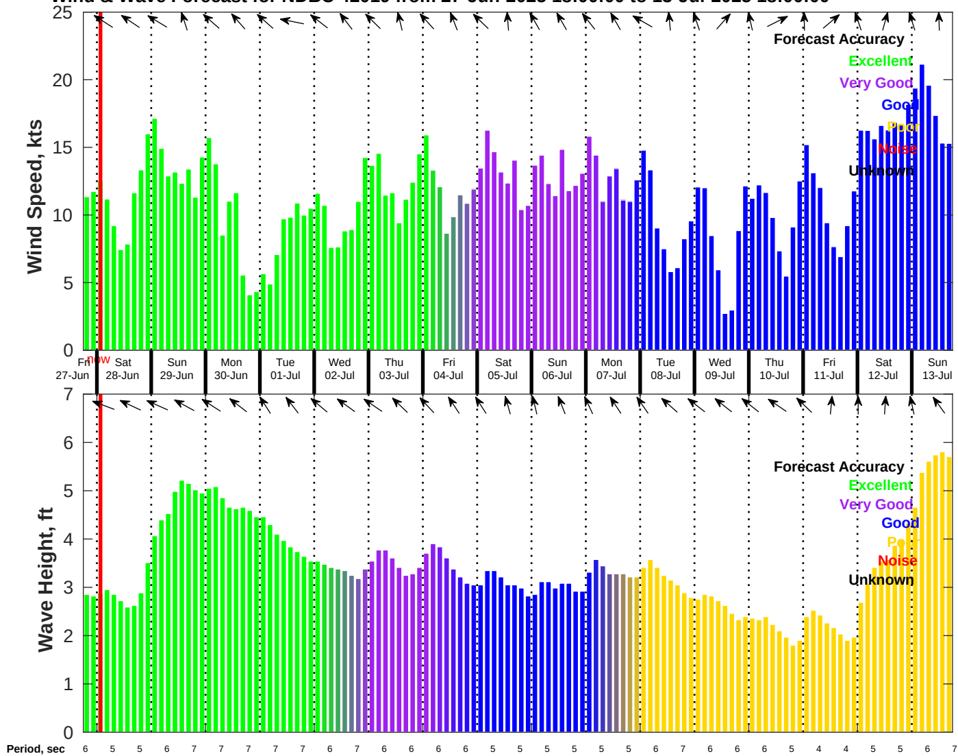
Wind & Wave Forecast for NDBC 42019 from 27-Jun-2025 18:00:00 to 13-Jul-2025 18:00:00
