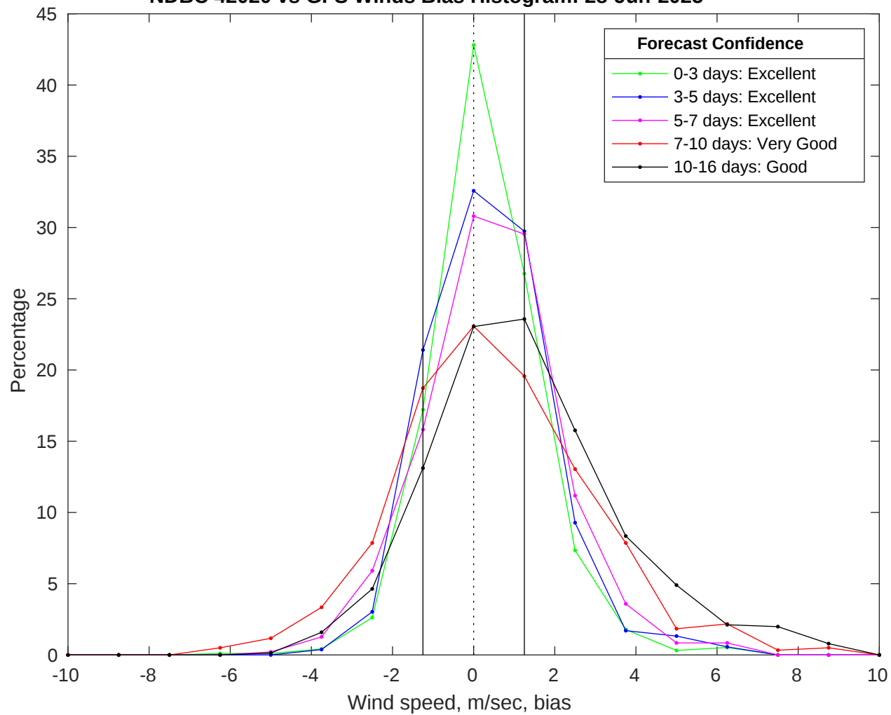
NDBC 42020 vs GFS Winds Bias Histogram: 28-Jun-2025
