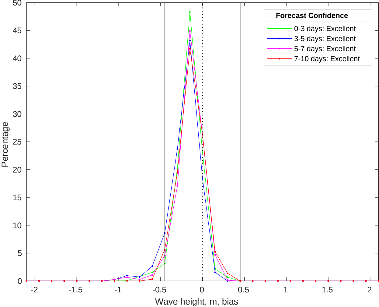
NDBC 42035 vs CMEMS Waves Bias Histogram: 28-Jun-2025
