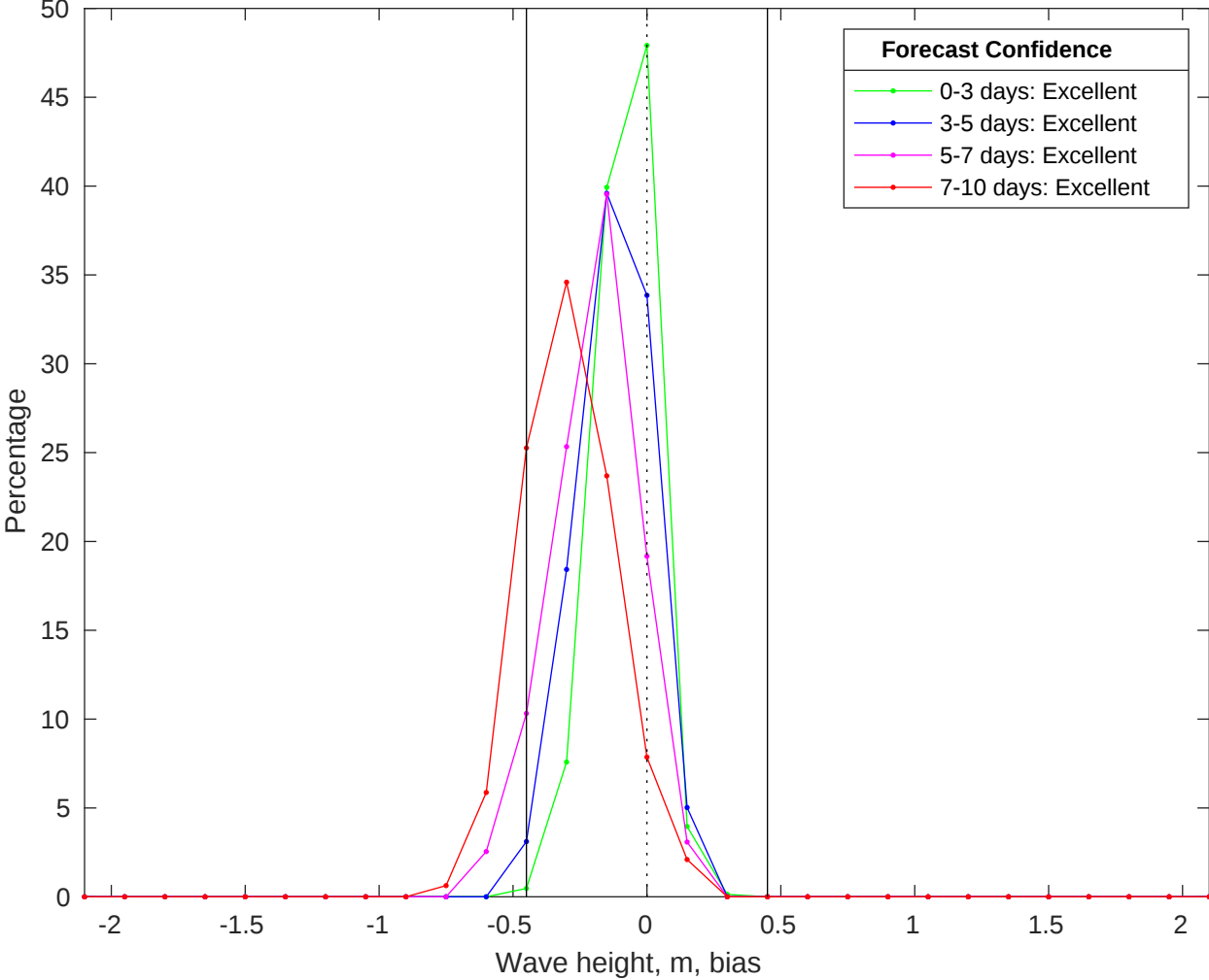
NDBC 42036 vs CMEMS Waves Bias Histogram: 28-Jun-2025
