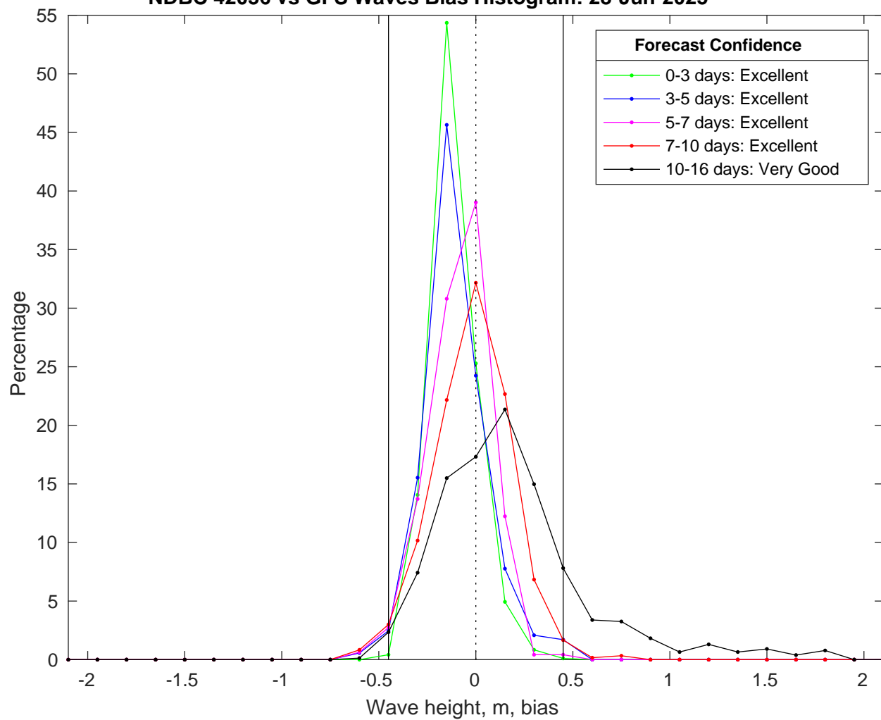
NDBC 42036 vs GFS Waves Bias Histogram: 28-Jun-2025
