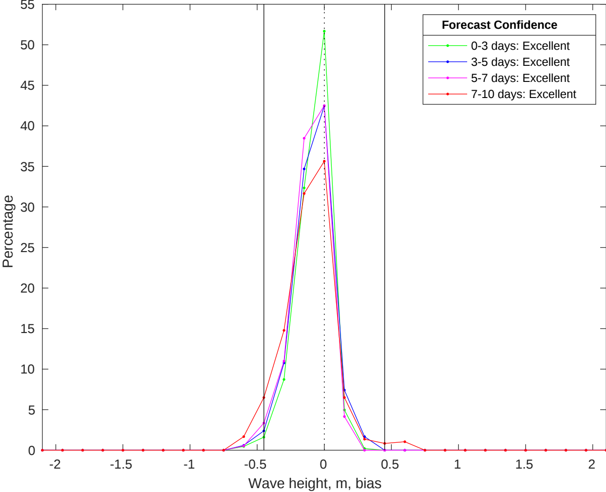
NDBC 42040 vs CMEMS Waves Bias Histogram: 28-Jun-2025
