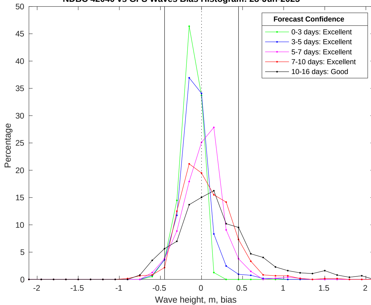
NDBC 42040 vs GFS Waves Bias Histogram: 28-Jun-2025
