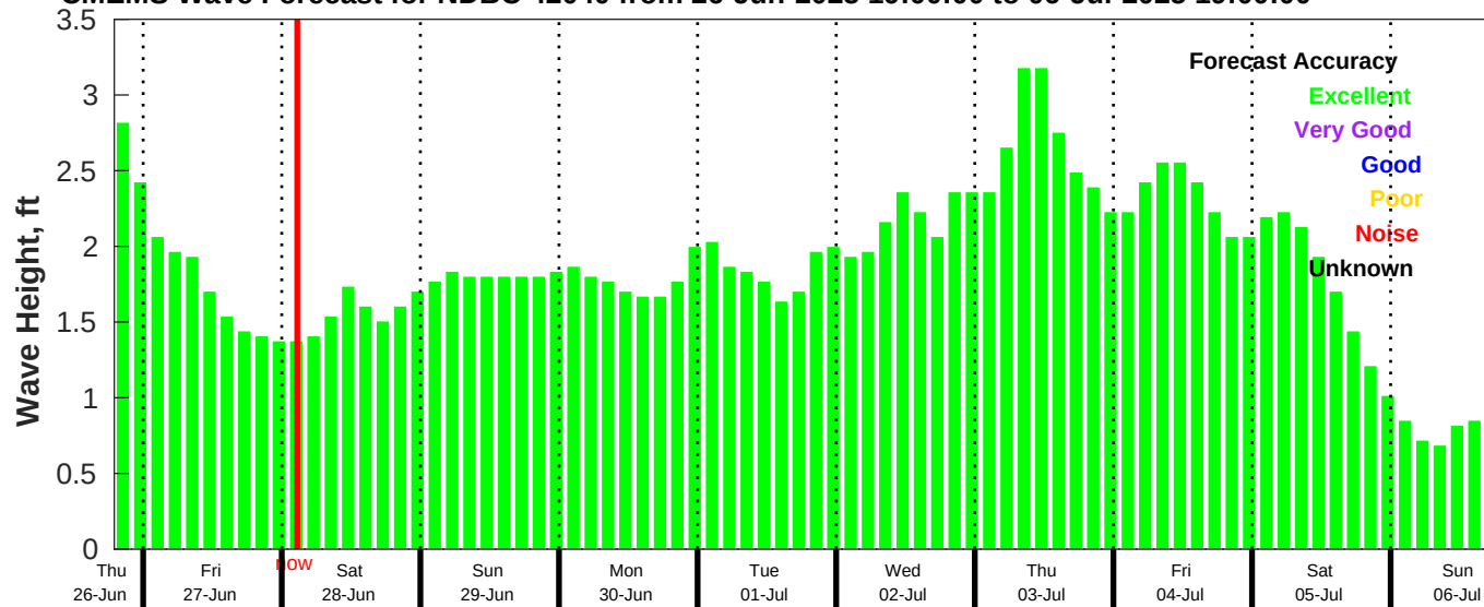
CMEMS Wave Forecast for NDBC 42040 from 26-Jun-2025 19:00:00 to 06-Jul-2025 19:00:00
