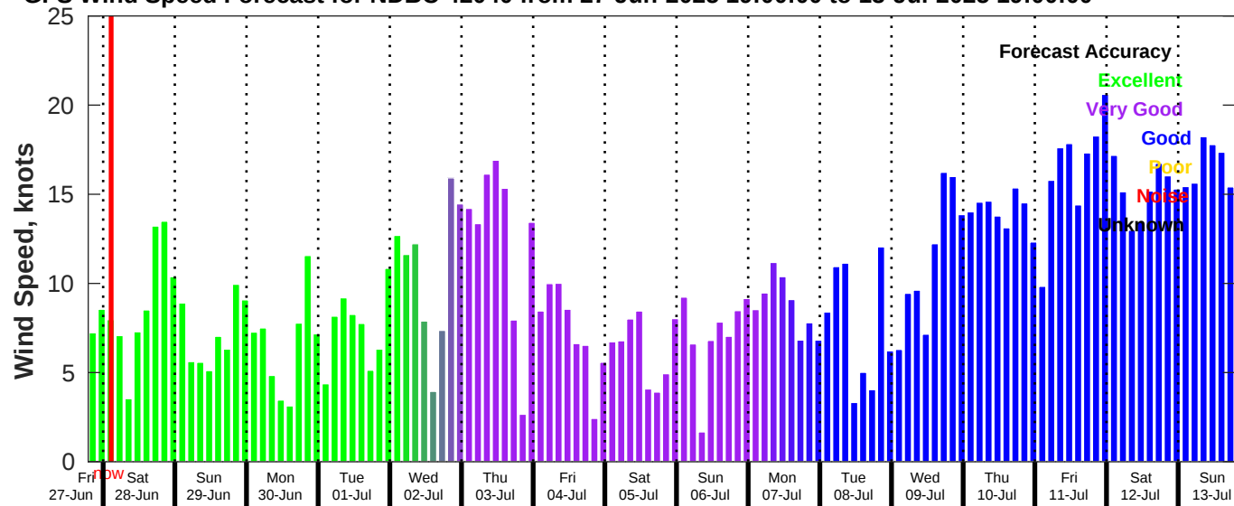
GFS Wind Speed Forecast for NDBC 42040 from 27-Jun-2025 19:00:00 to 13-Jul-2025 19:00:00
