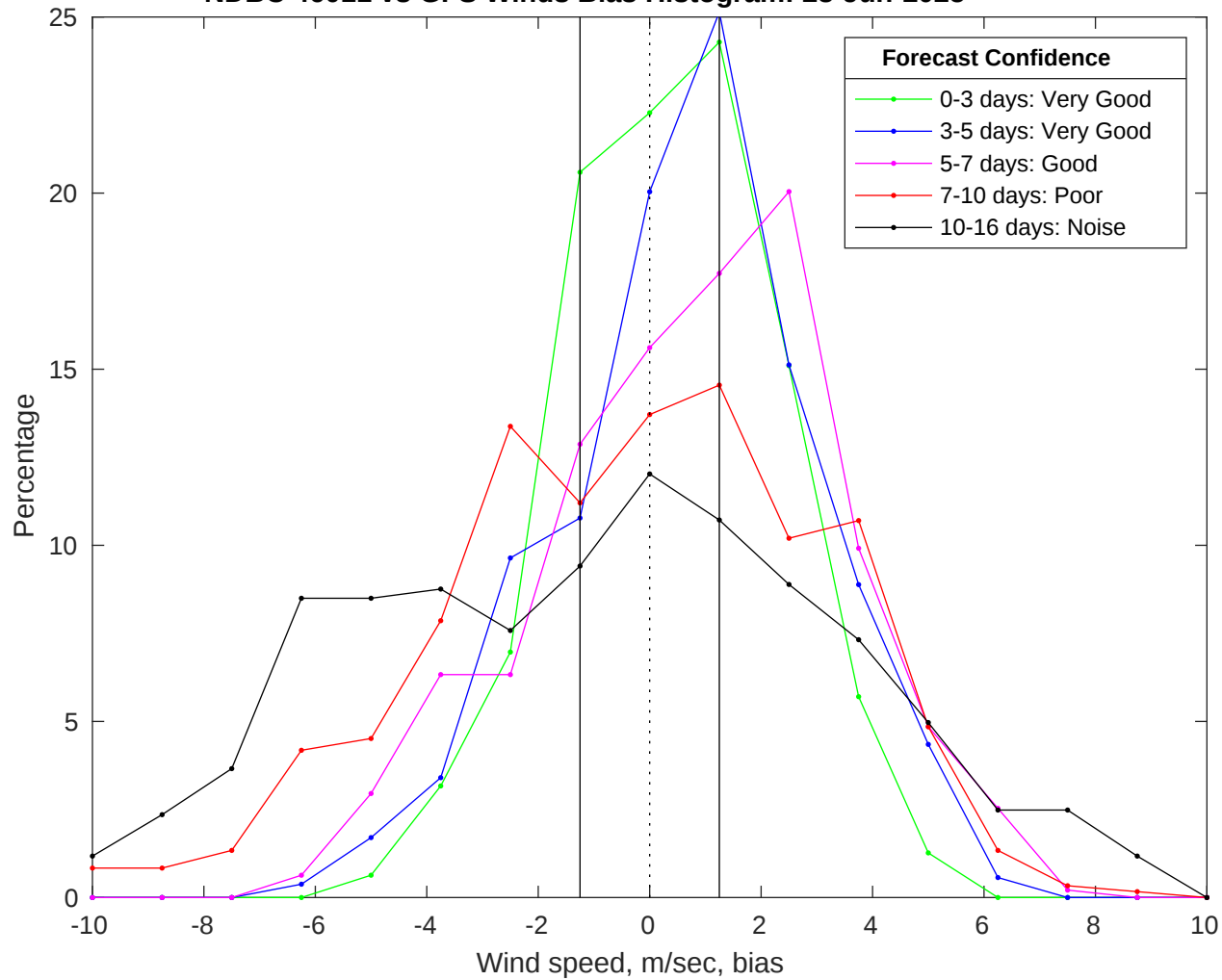
NDBC 46011 vs GFS Winds Bias Histogram: 28-Jun-2025
