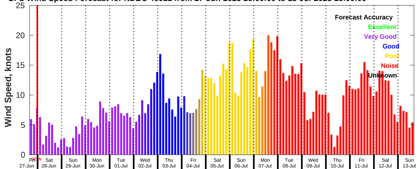
GFS Wind Speed Forecast for NDBC 46011 from 27-Jun-2025 16:00:00 to 13-Jul-2025 16:00:00
