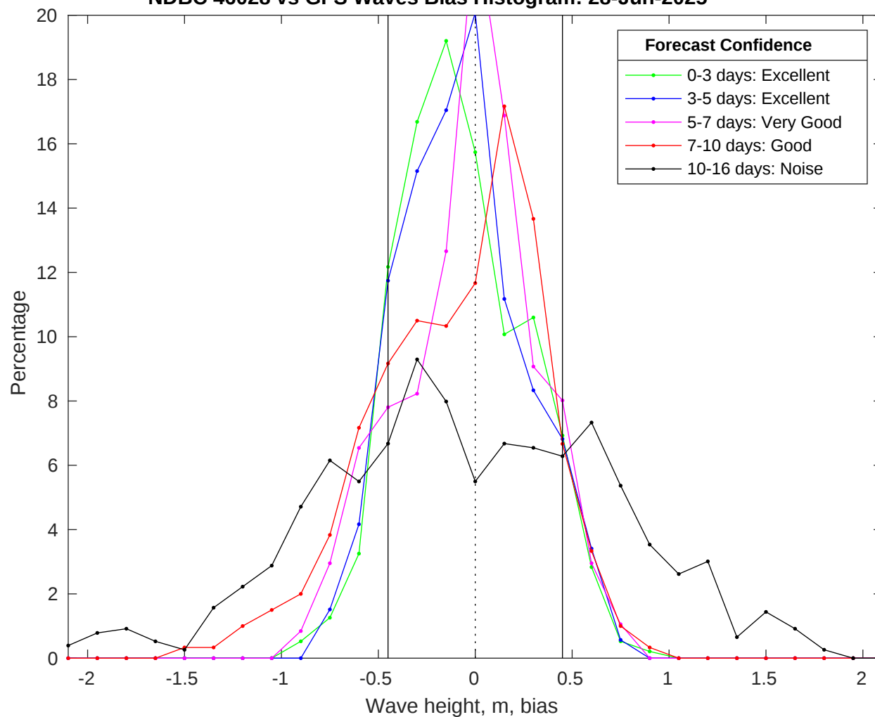
NDBC 46028 vs GFS Waves Bias Histogram: 28-Jun-2025
